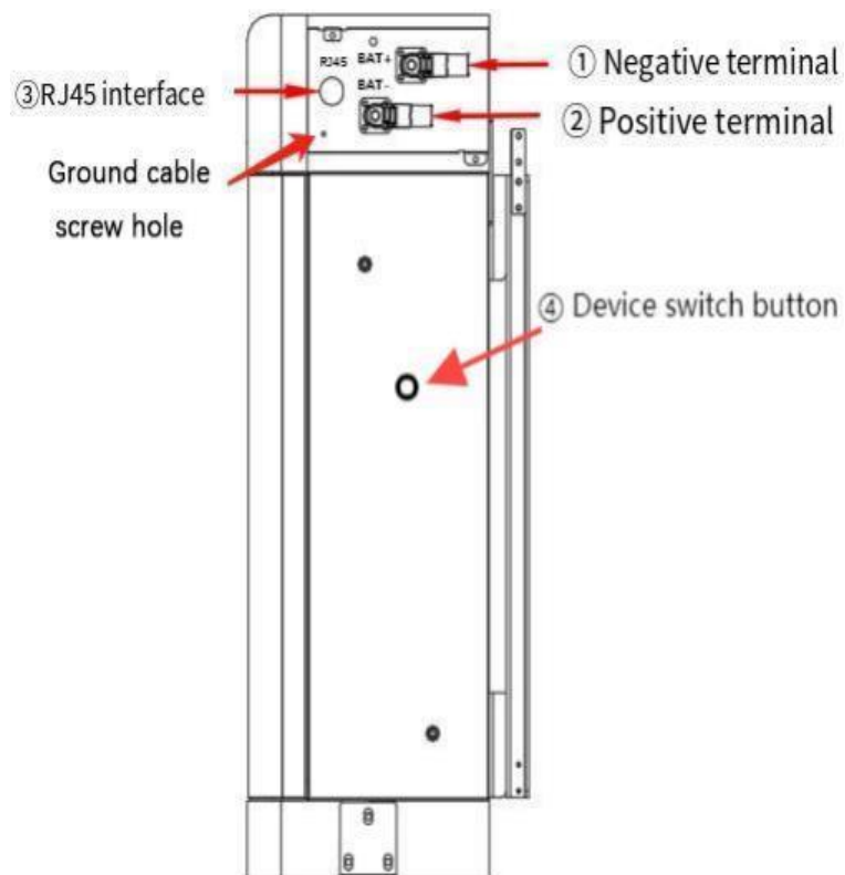
Figure1-3 Structure of the INNO-A-5kW Series
